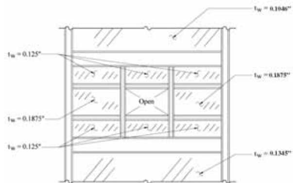
Fig. 6–6. SPSW panel with opening.
