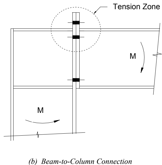
Figure 1-2 Typical uses of end-plate moment connections (extended).
